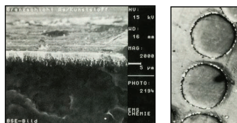
Cross section views of nylon fiber showing silver deposits
