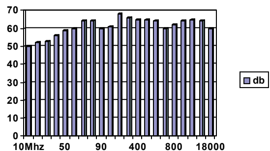
Nanking Conductive Fabric Tape Mil-Std 285 Modified
